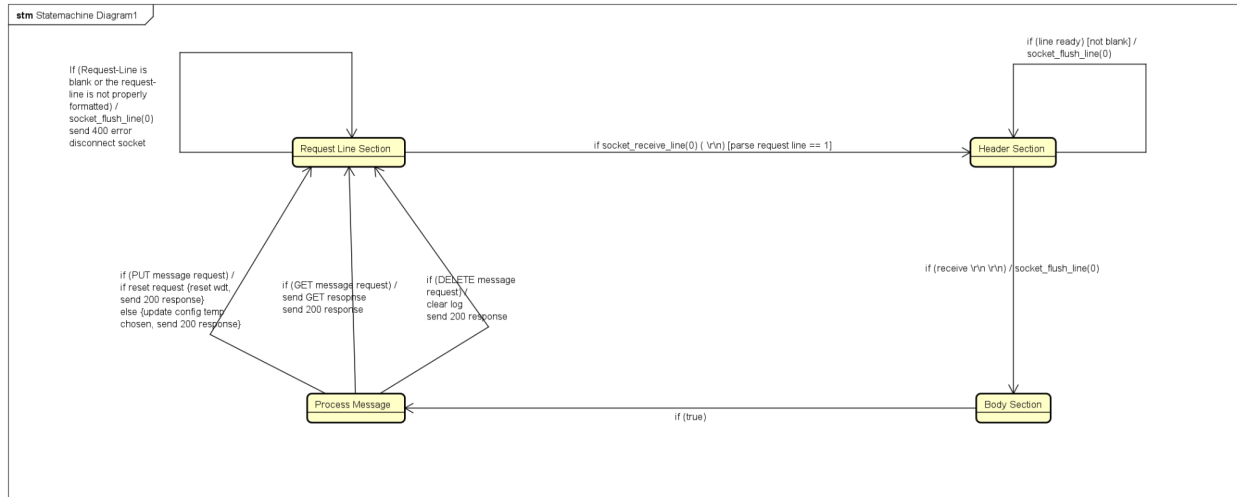
Figure 1. HTTP Parser FSM - The diagram illustrates a UML state machine for parsing incoming HTTP requests. The FSM contains four states: Request Line Section, Header Section, Body Section, and Process Message. The FSM starts in the Request Line Section and waits for a complete line in the socket receive buffer. A blank or malformed request line causes the FSM to flush the buffer, send a 400 error, disconnect, and remain in the Request Line Section. A valid request line advances the FSM to the Header Section. The Header Section discards incoming header lines until a blank line signals the end of the HTTP header block, at which point the FSM advances to the Body Section. The Body Section passes through immediately to Process Message, as all supported endpoints use query string parameters rather than a request body. In Process Message, the FSM dispatches based on the parsed method and URI, sends the appropriate response, disconnects the socket, and resets to the Request Line Section to await the next request.
